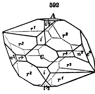
Brewster.
